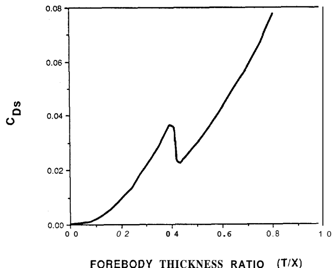
Fig. 6. Relationship between spray component of drag, C_{Ds} , and Forebody Thickness Ratio. Modified from Hoerner, 1965.
