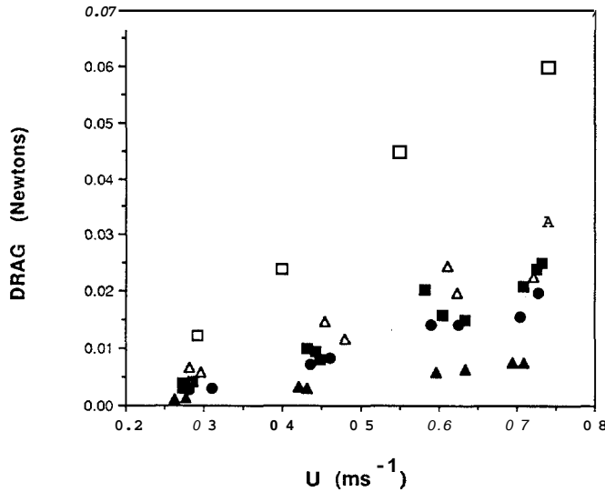
Fig. 2. Drag on isolated hind feet as a function of the water velocity, U . Open symbols represent the fishing bats, Noctilio leporinus ( \square ) and Pizonyx vivesi ( \Delta ); closed symbols represent non-fishing bats, Myotis velifer ( \blacktriangle ), Noctilio albiventris ( \blacksquare ), and Pteronotus parnellii ( \bullet ).
